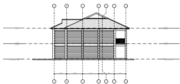
ELEVATION E-03
